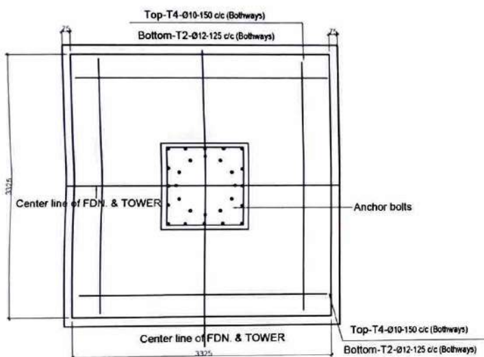
SECTIONAL PLAN
