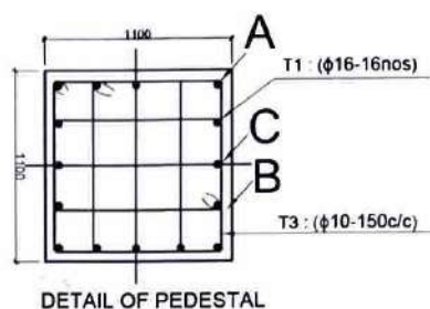
DETAIL OF PEDESTAL
