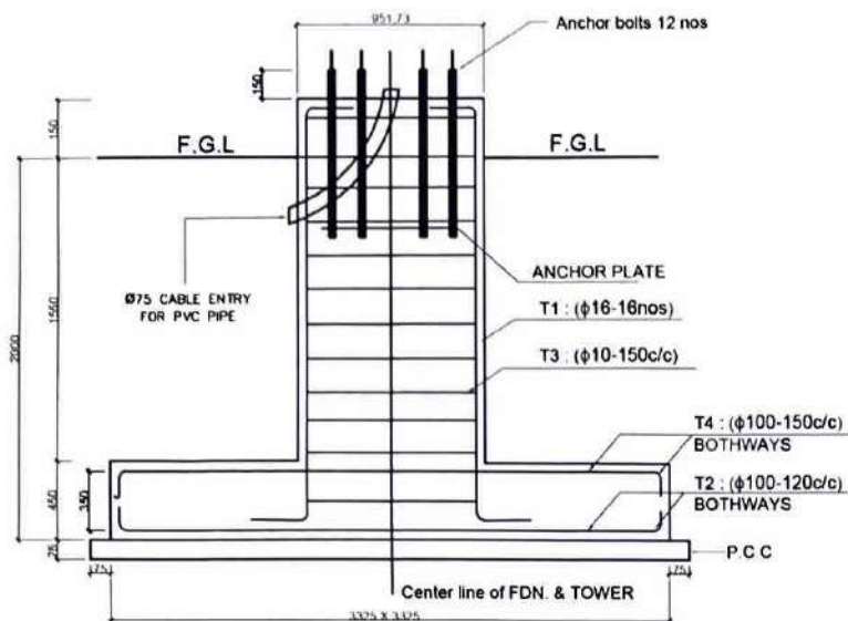
SECTIONAL ELEVATION
